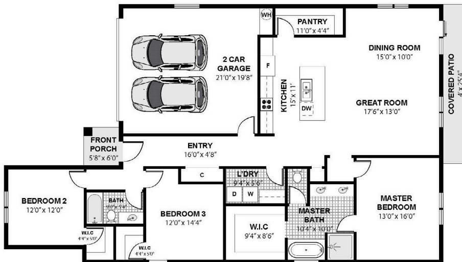
MAIN FLOOR
